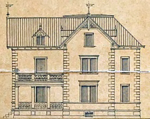
OSTFACADE.
