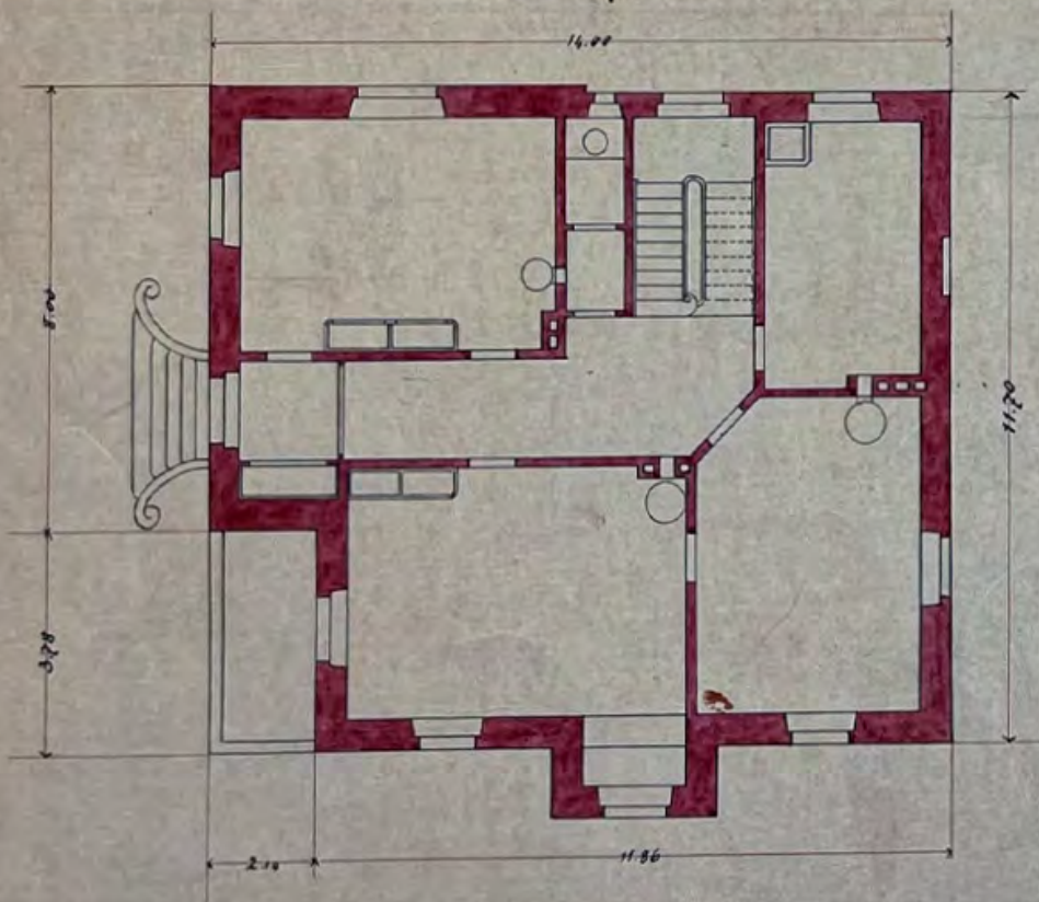
Erdgeschoss.
